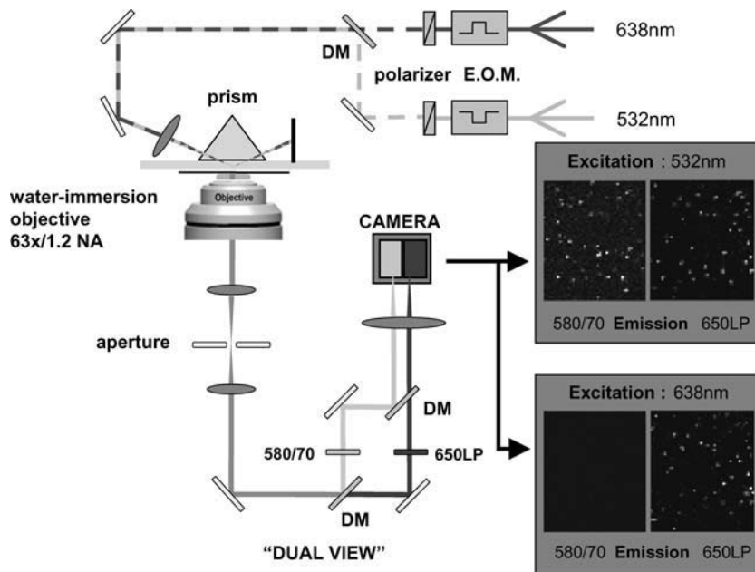
FIGURE 2 msALEX-DI, experimental setup; EOM, electrooptic modulator; DM, dichroic mirror. The image is split into two zones on the CCD camera, corresponding to the donor (left) and the acceptor (right) emission channels. The camera is synchronized with the alternation of the lasers, resulting in four images of the illuminated area (two excitations \times two emissions).
